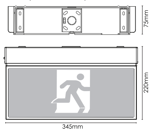
EXS-EDGE (Surface Mounted):
